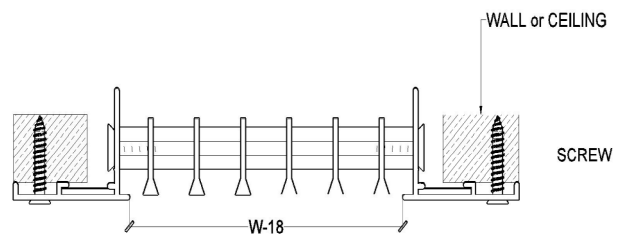
Screw
