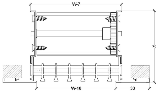
LINEAR BAR GRILLE SUPPLY
